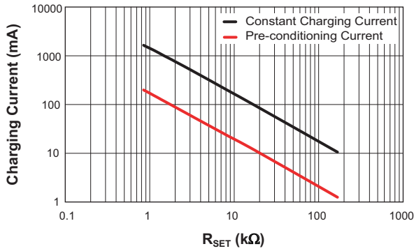
Charging Current vs. Set Resistor Values
